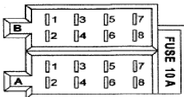
FIXED ISO SOCKET SKETCH
